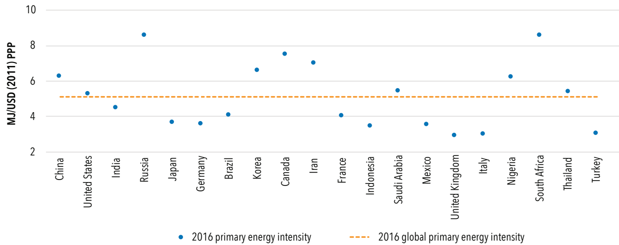
FIGURE 4.6 • PRIMARY ENERGY INTENSITY IN THE 20 COUNTRIES WITH THE LARGEST TOTAL PRIMARY ENERGY SUPPLY, 2016
